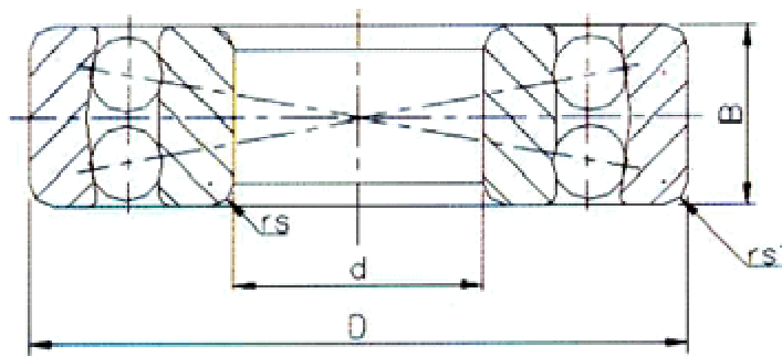
Self-aligning ball bearings of cylindrical bore10000
