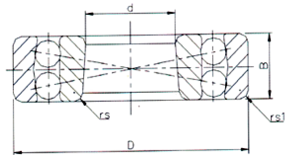
Self-aligning ball bearings of tapered bore10000K
